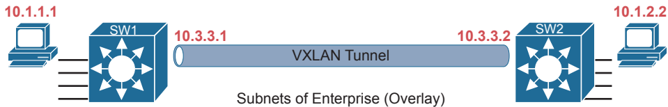
Figure 17-7 VXLAN Tunnel and Endpoints with IPv4 Addresses in the Same IPv4 Space
