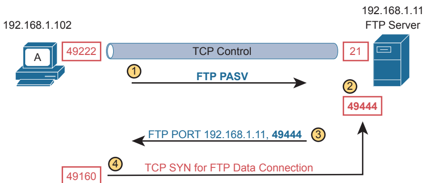
Figure 12-19 FTP Passive Mode Process to Create the Data Connection
