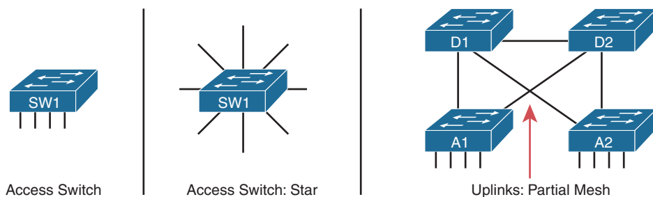
Figure 13-6 LAN Design Terminology
