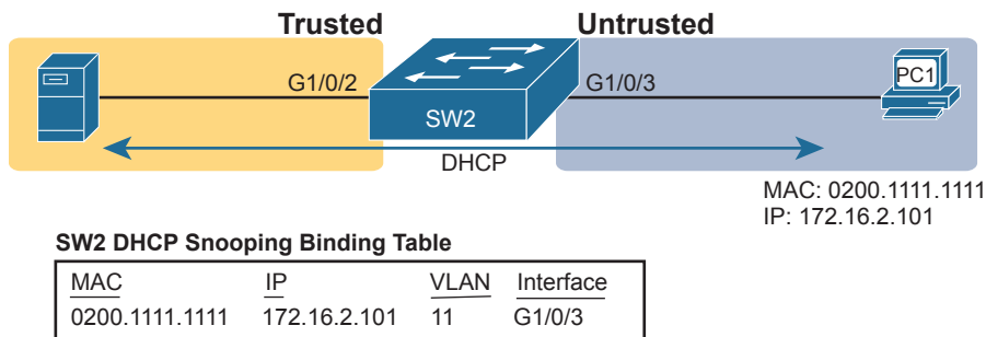
Figure 8-6 Legitimate DHCP Client with DHCP Binding Entry Built by DHCP Snooping
