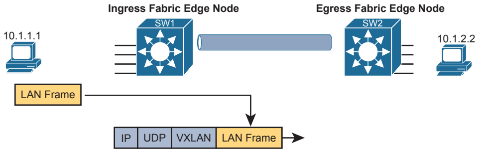
Figure 17-5 Fundamentals of VXLAN Encapsulation in SDA
